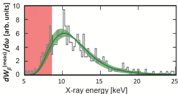
FIG. 15 Color online. Measured betatron radiation spectrum dW_{\beta}^{(meas)}/d\omega (solid black histogram) used to determine beam radius \sigma_r inside LWFA that produced a peaked electron energy spectrum similar to the one shown in Fig.11b. Solid green curve: calculated spectrum dW_{\beta}/d\omega , assuming \sigma_r \lesssim r_{\beta} = 0.8 \mu\text{m} . Shaded green area: variation in dW_{\beta}/d\omega for 25% variation in \sigma_r . Red-shaded area (5 – 8 keV): low-energy regime with reduced detection efficiency and measurement quality. Experimental conditions matched those of (Couperus et al. , 2017; Köhler et al. , 2016).
