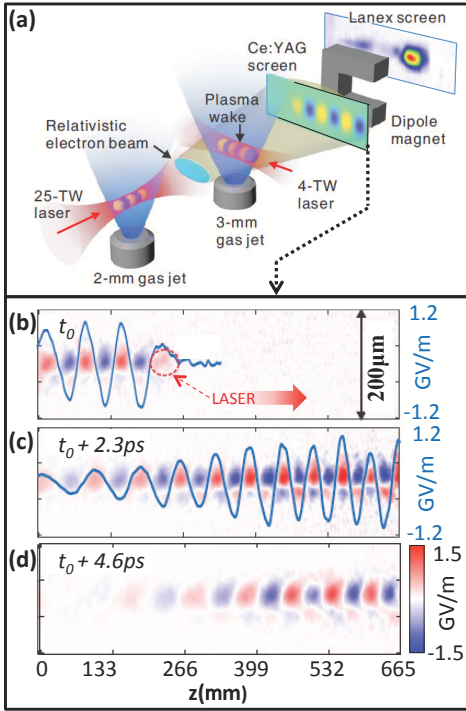
FIG. 34 Color online. Transverse electron radiography of laser wakefield. (a) Schematic experimental setup. The electron probe bunch (4 fs FWHM, 2-10 pC, 7 mrad FWHM divergence) from one plasma accelerator (2mm gas jet, \bar{n}_e = 8 \times 10^{18} \text{ cm}^{-3} , 95% He, 5% N 2 ) driven by a 25 TW, 40 fs FWHM Ti:S laser pulse, propagates transversely through the “subject” plasma accelerator (3mm gas jet, with synchronized 4 TW, 100 fs FWHM Ti:S drive pulse) located 11 cm away, then exposes a Ce:YAG scintillator further downstream. Magnetic spectrometer can measure probe bunch energy with scintillator removed. From (Zhang et al. , 2017). Below: scintillator images at probe delays (b) t_0 , (c) t_0 + 2.3 \text{ ps} , and (d) t_0 + 4.6 \text{ ps} of wake generated in tapered density up-ramp ( \bar{n}_e \approx 2.5 \times 10^{17} \text{ cm}^{-3} at z = 0 to 3.5 \times 10^{17} \text{ cm}^{-3} at z = 665 \mu\text{m} ), yielding decreasing plasma period evident in panels (b), (c). Panels b) thru d) from (Zhang et al. , 2018).
